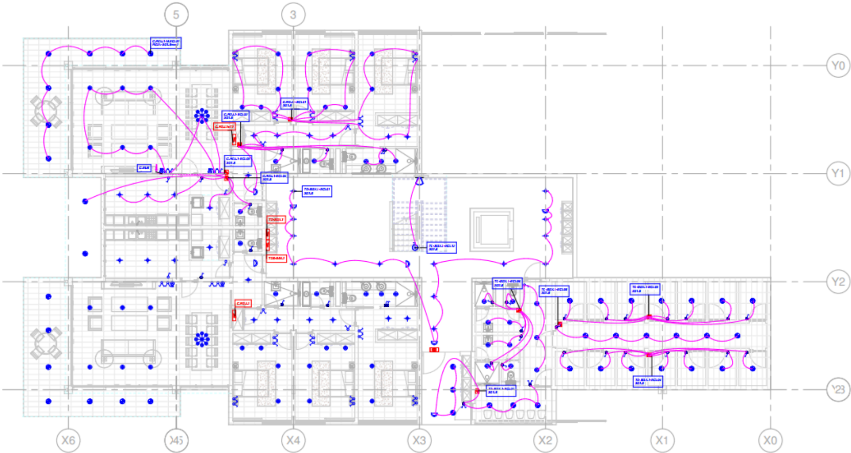
PLAN ECL RDJ
