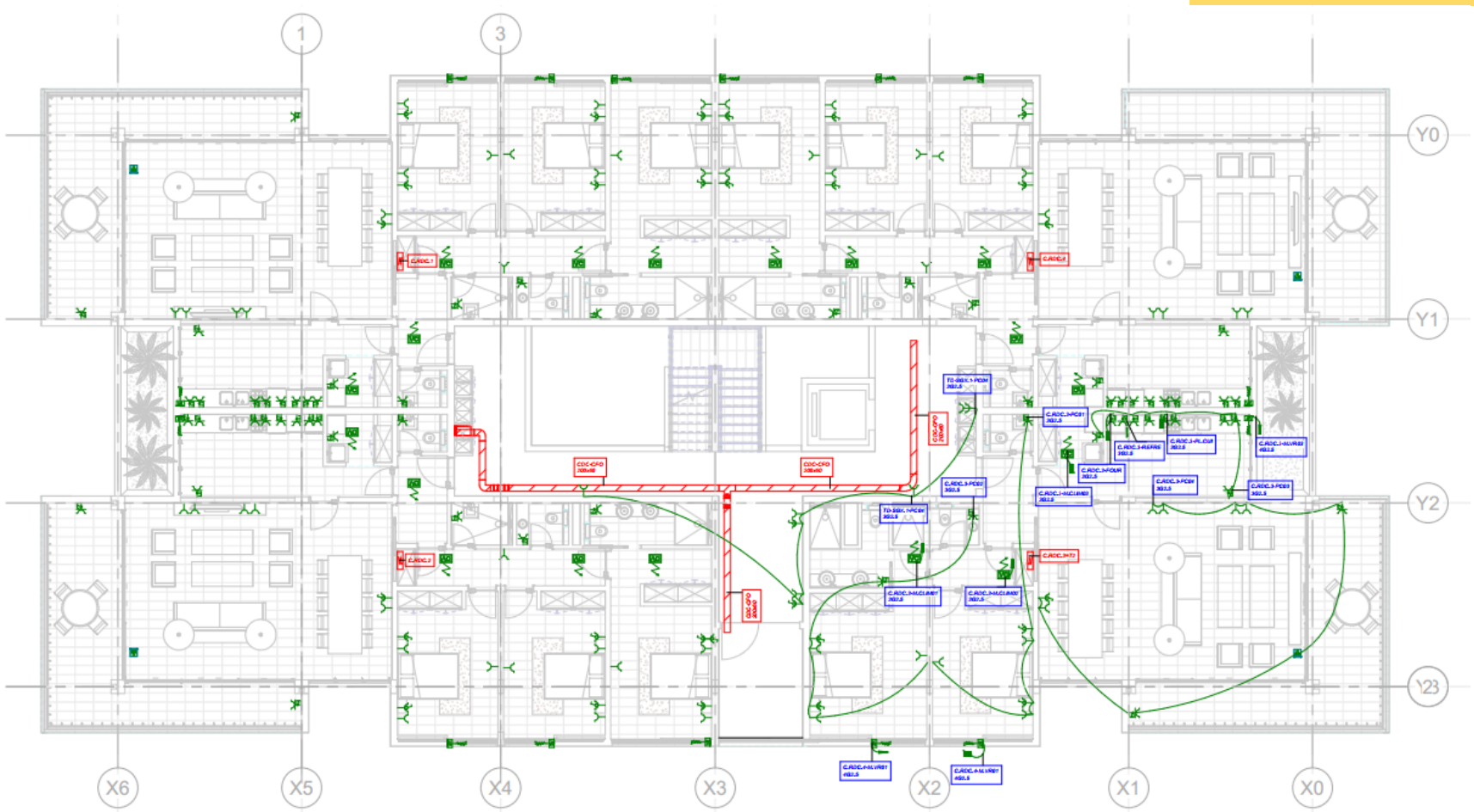
PLAN CFO RDC/ET1/ET2
