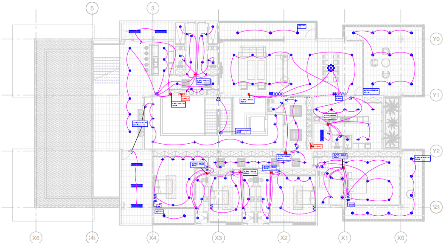
PLAN ECL PENTHOUSE
