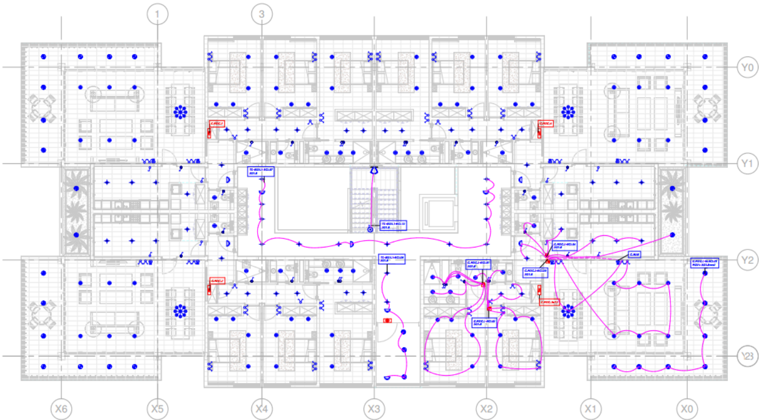
PLAN ECL RDC/ET1/ET2
