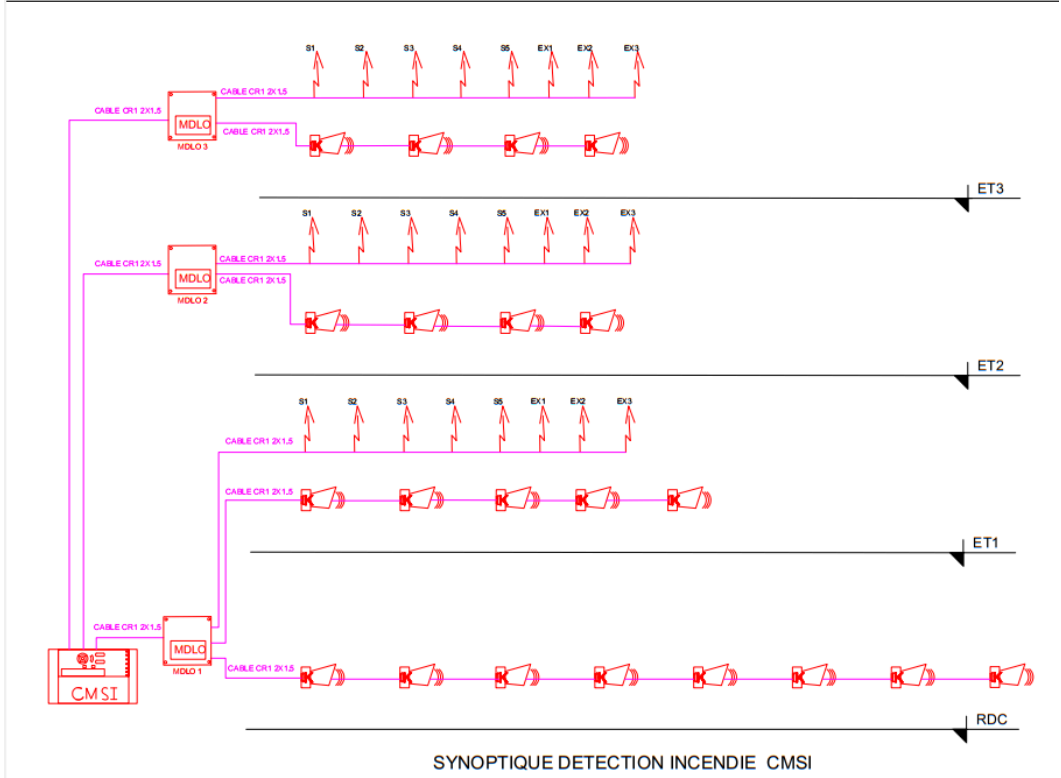
SYNOPTIQUE DETECTION INCENDIE
